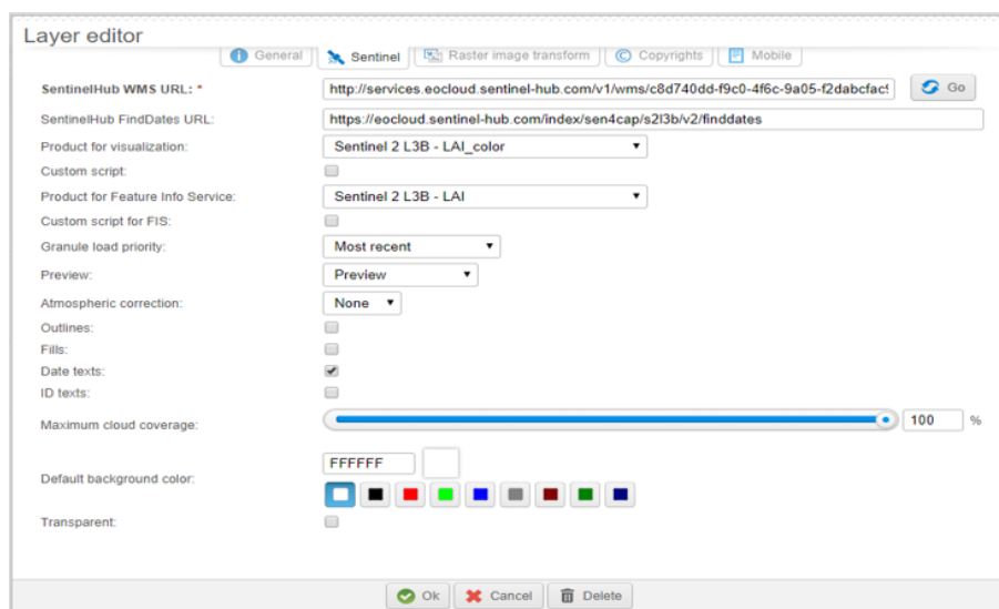
Figure 6-9. Settings for the S2 L3A - LAI layer
