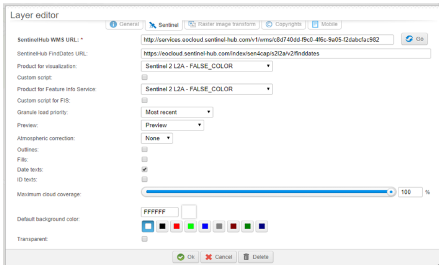
Figure 6-7. Settings for the S2 L2A False Color layer
