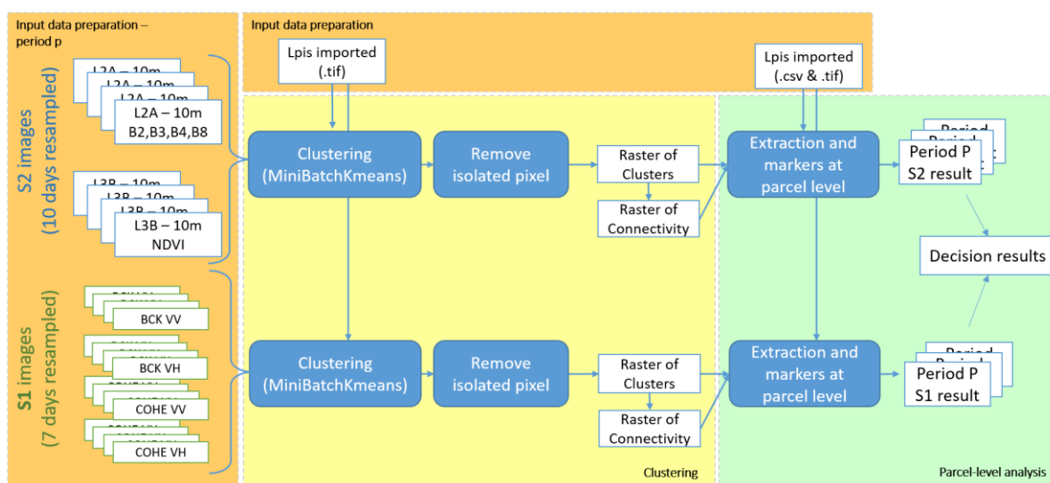
Figure 2-6 - General workflow of the L4D heterogeneity detection algorithm
