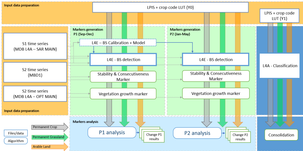
Figure 2-8 - General workflow of the L4F category change algorithm
