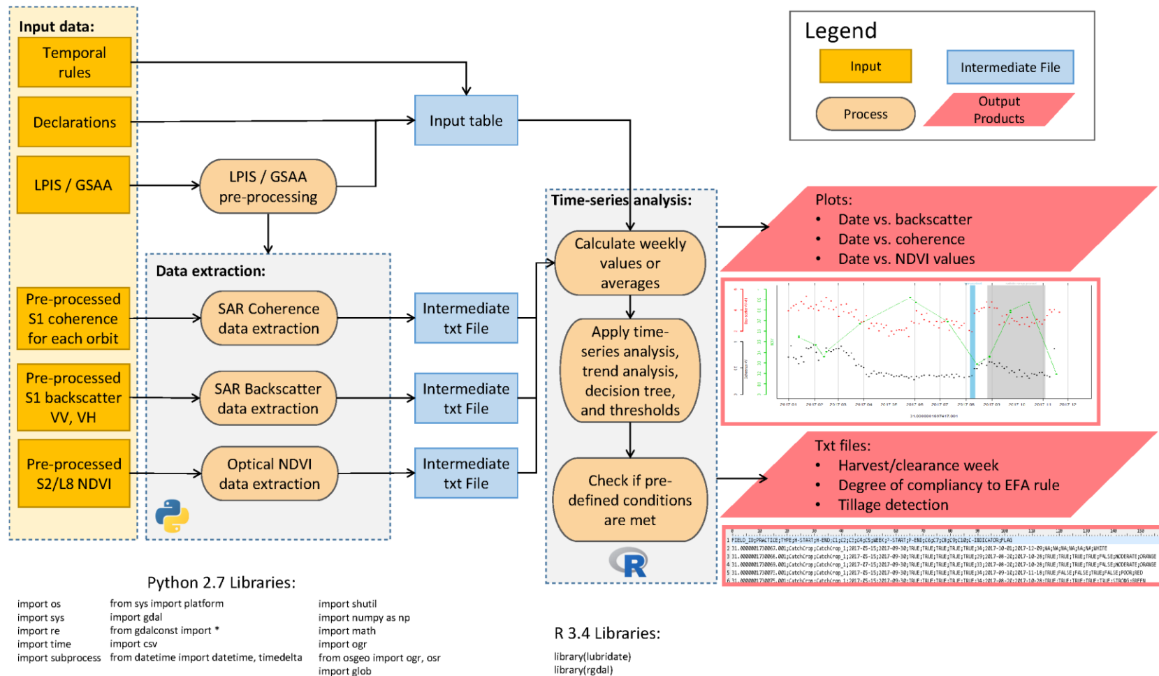
Figure 2-5. Logical data flow of the LAC agricultural practices monitoring product
