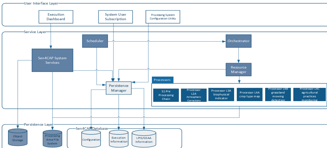
Figure 2-9. Software System Architecture
