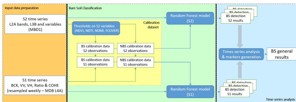
Figure 2-7 - General workflow of the L4E bare soil detection algorithm
