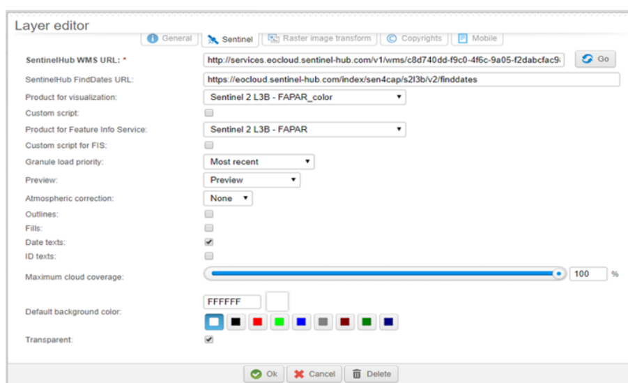
Figure 6-10. Settings for the S2 L3A - FAPAR layer
